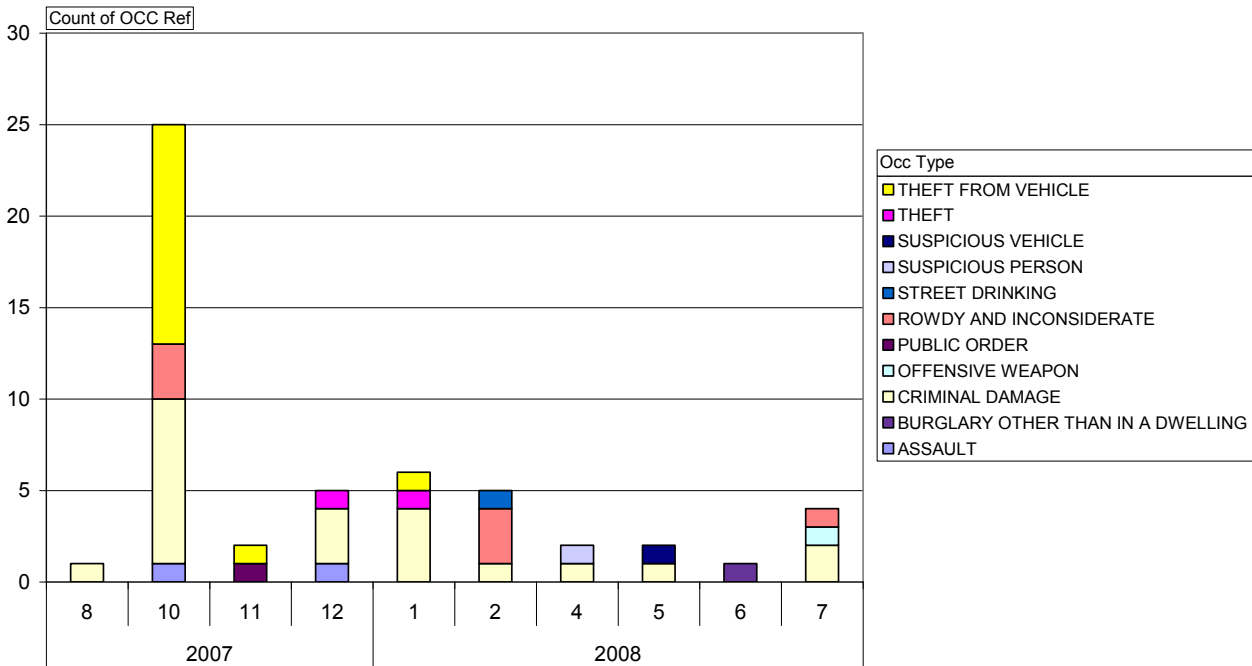
Figure 2 – Incidents subjectively decided by the analyst to be plausibly linked to The George, by month and Occurrence type, (1/7/07-10/8/08)
